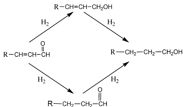
Scheme 2 Transformation of the α,β-unsaturated aldehydes.
