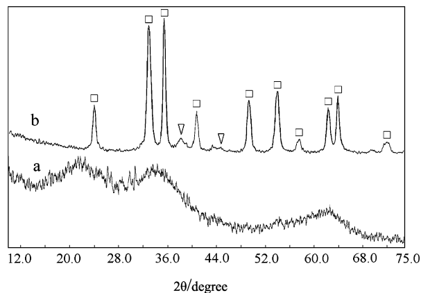
Fig. 2 X-Ray diffraction patterns for supported Au catalysts: (a) 1.0 wt% Au/Fe(OH) x , (b) 1.1 wt% Au/Fe 2 O 3 -4. (□) hematite; (▽) metallic gold.
