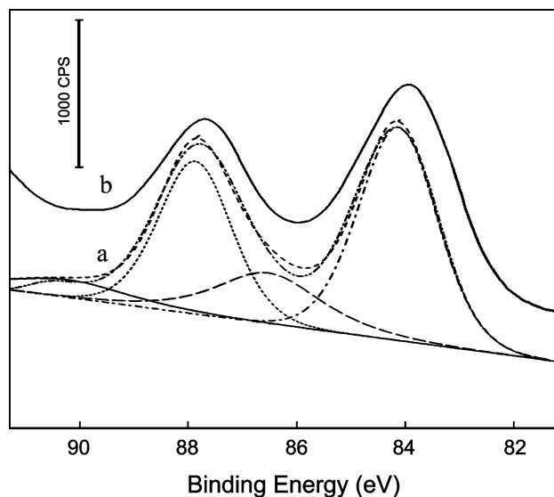
Fig. 3 XPS spectra of supported Au catalysts: (a) 1.0 wt% Au/Fe(OH) x , (b) 1.1 wt% Au/Fe 2 O 3 -4.
