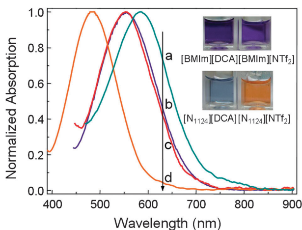
Fig. 3 Longest wavelength intramolecular charge-transfer \pi - \pi^* absorption bands of Reichardt's betaine dye 30 in [N 1124 ][DCA] (a), [BMIm][NTf 2 ] (b), [BMIm][DCA] (c) and [N 1124 ][NTf 2 ] (d). Inset is a photograph illustrating the appearance of IL solutions of Reichardt's dye 30.
